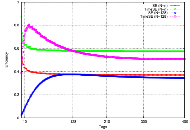
Fig. 2. System efficiency and time system efficiency for FSA protocol.
